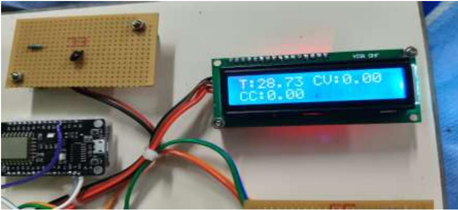
(a) Monitoring of Battery Temperature
