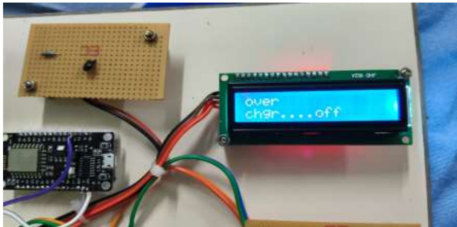
(c) Over charge Alert
